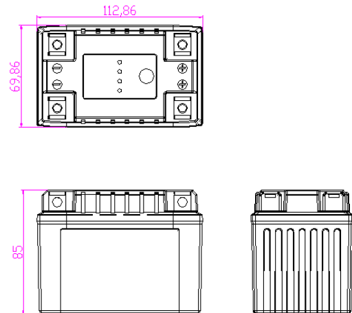
Dimensions (mm)
