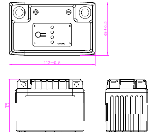
Dimensions (mm)
