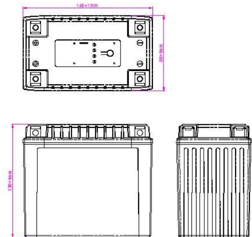
Dimensions (mm)
